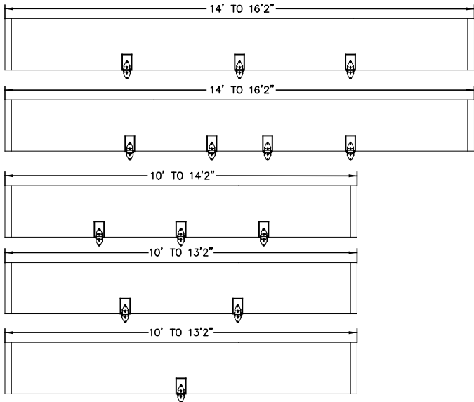
HINGE & BACKER PLATE LOCATIONS
